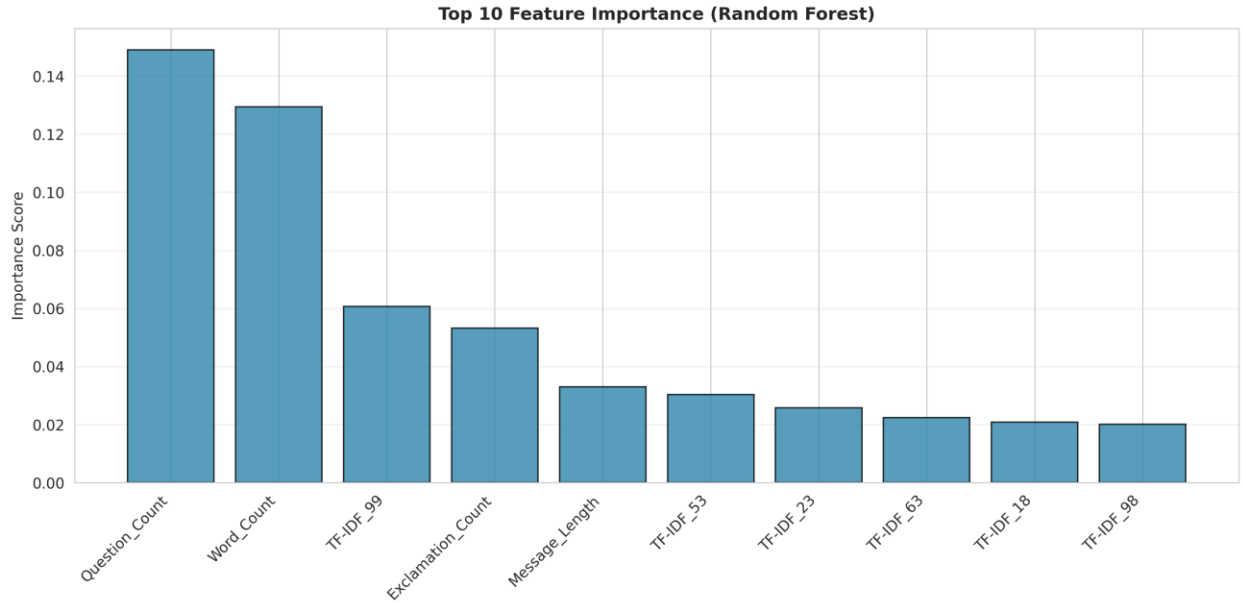
Figure 5: Top 10 Feature Importance (Random Forest)
