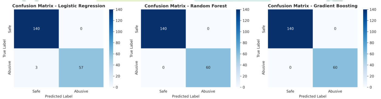
Figure 3: Confusion Matrices for Classification Models
